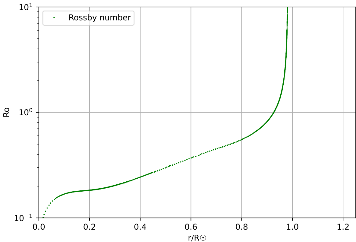
Rossby number, profile 145, age 4.2 \times 10^9
